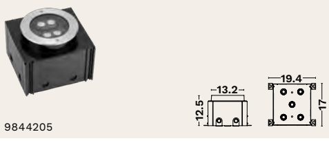
MOUNTING SLEEVE
