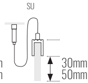
Sarkıt. Suspended
